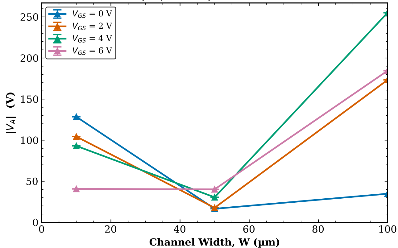
TFT3 Transistor 2 |V_A| vs W | L = 20\text{ }\mu\text{m}
